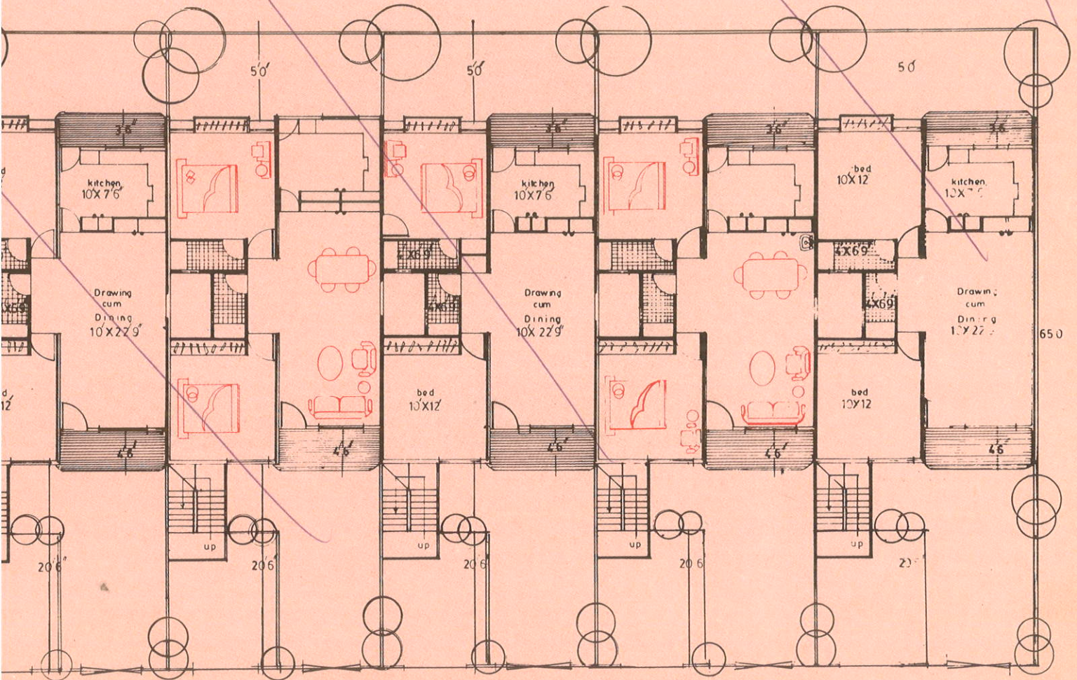
PLAN TYPE II & III A, B
