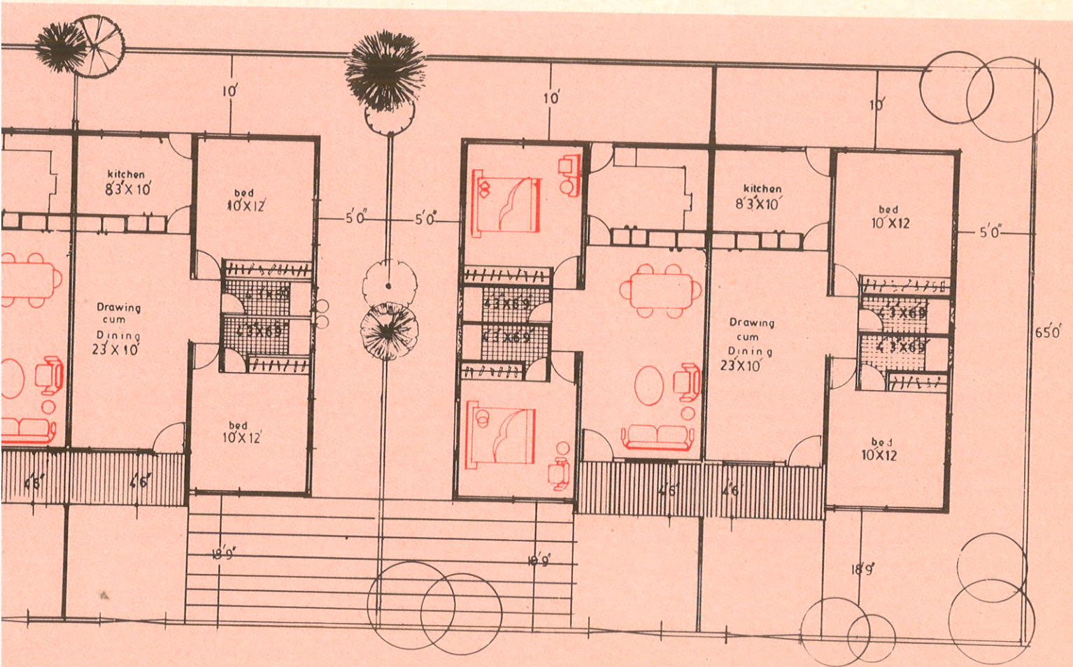
PLAN TYPE I
